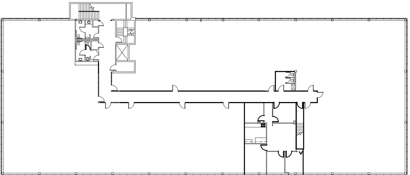
WEST BUILDING - THIRD FLOOR SCALE: 1/8"=1'-0"
